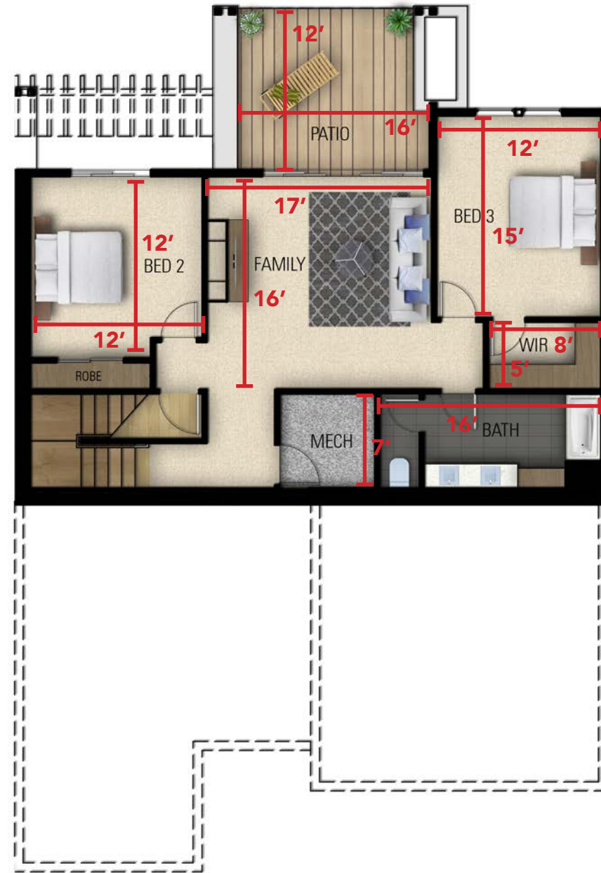
Lower Floor Plan
